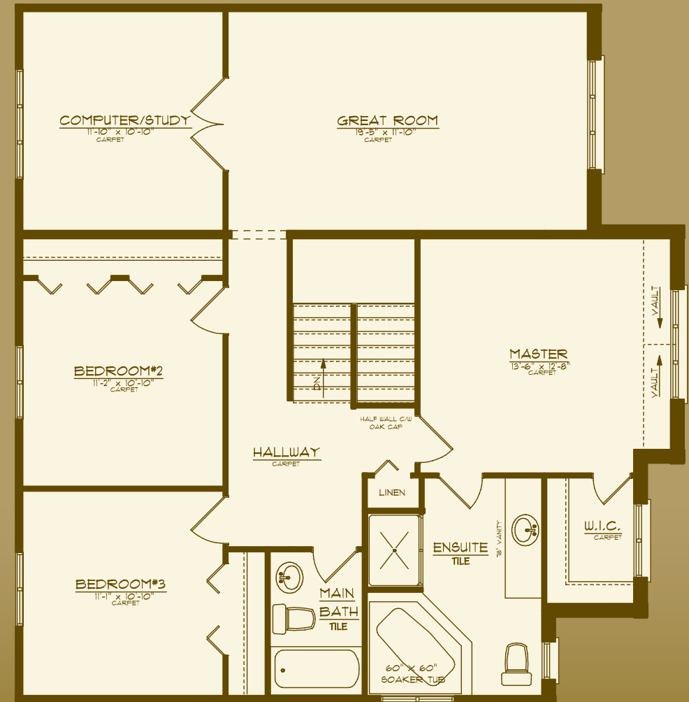
Upper Floor 1,279 Sq. Ft.
